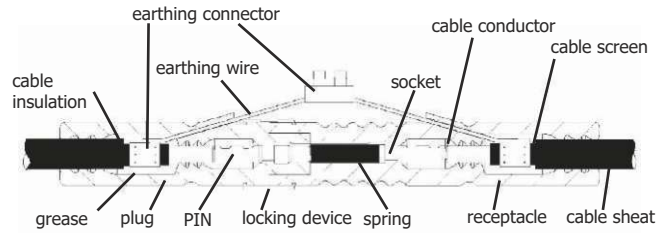
KD 500 (screened cable)
